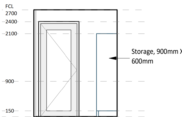
5 ELEVATION DETAIL 60-020 1 : 50
