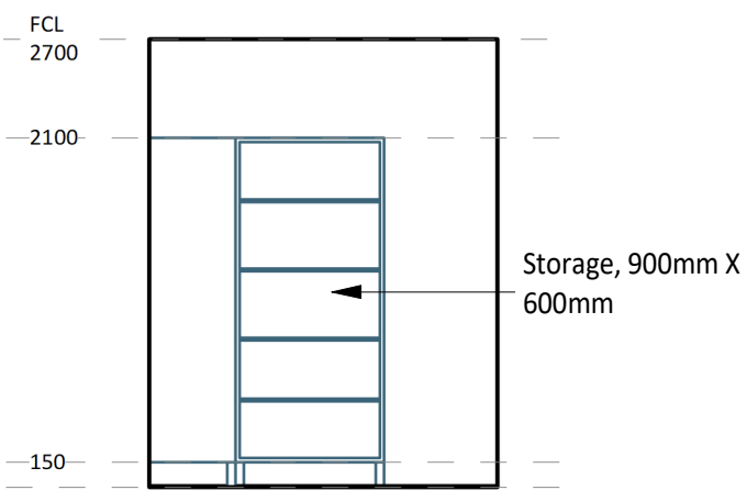
3 ELEVATION DETAIL 60-025 1 : 50
