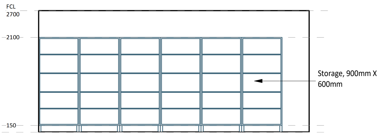
2 ELEVATION DETAIL 60-020 1 : 50
